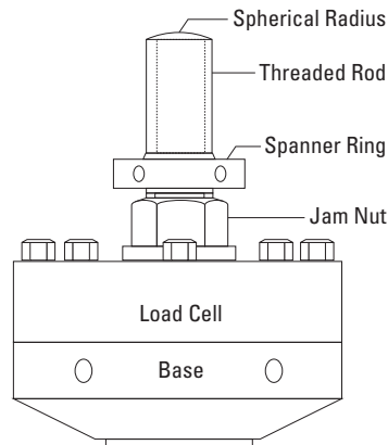
Figure 51. Load Cell with Calibration Adapter Installed.
