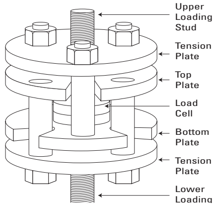
Figure 88. Compression Gage
