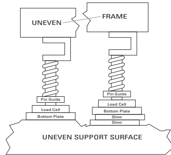
Figure 73. Shimming a Springy System
