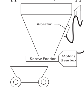
Figure 80. Optimizing Conduit Loading
